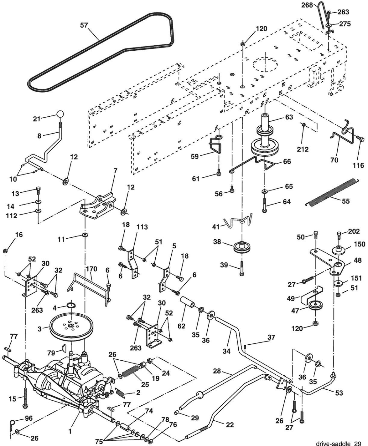
drive-saddle_29
