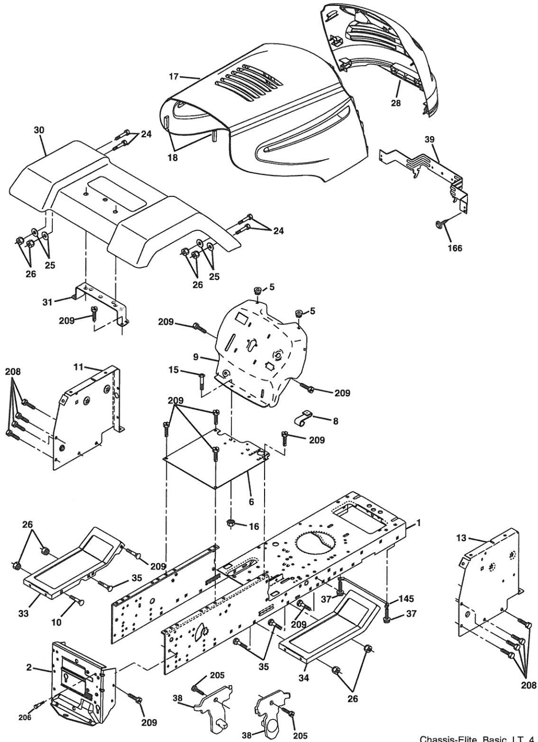
Chassis-Elite_Basic_LT_4
